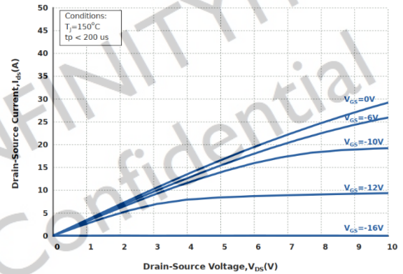
Figure 2 Typical Output Characteristics T_j = 150^\circ\text{C} (Parameter : V_{GS} )
