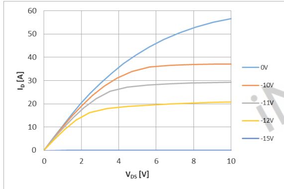
Figure 1 Typical Output Characteristics T_j = 25\text{ }^{\circ}\text{C} (Parameter : V_{GS} )
