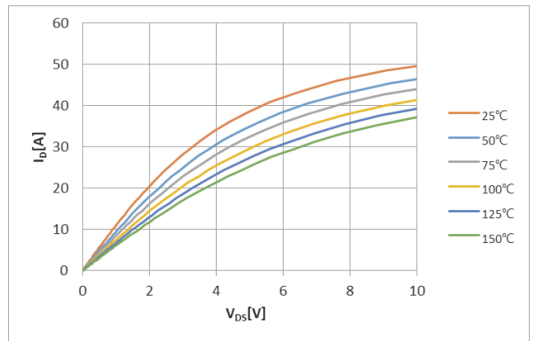
Figure 8. Characteristics for various temperatures Parameter: T_J
